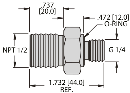
PCV-N1/2A4 | M6835013
