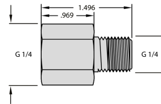
Pressure Snubber
