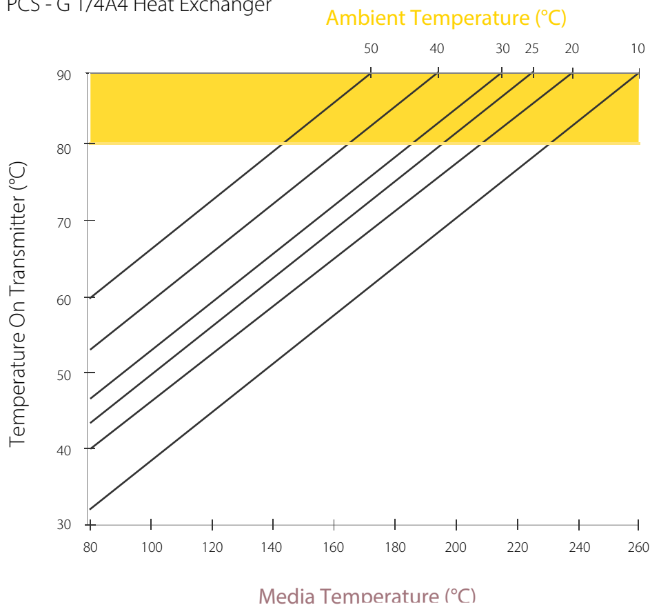
PCS - G 1/4A4 Heat Exchanger
