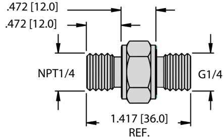
PCV-N1/4A4 | A9867
