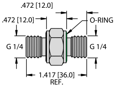
PCV-G1/4A4 | M6835011
