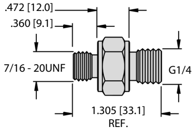
PCV-S7/16A4 | A9136
