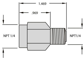
Pressure Snubber
