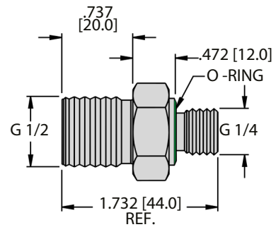
PCV-G1/2A4 | M6835012
