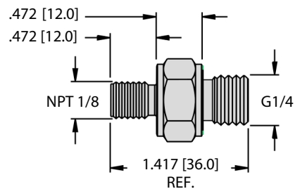
PCV-N1/8A4 | M6835021
